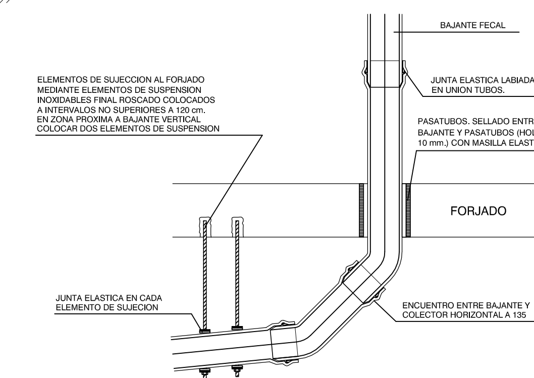
DETALLE SUSPENSION COLECTORES - (SECCION)
